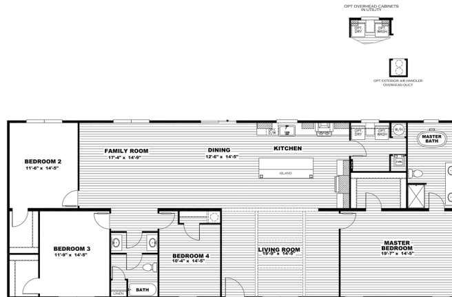
MODEL #PCH32764A DRAWING # 30M007 32'X76' THE COLUMBUS
